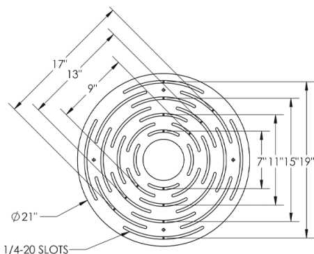
MOUNTING PLATE DETAIL
