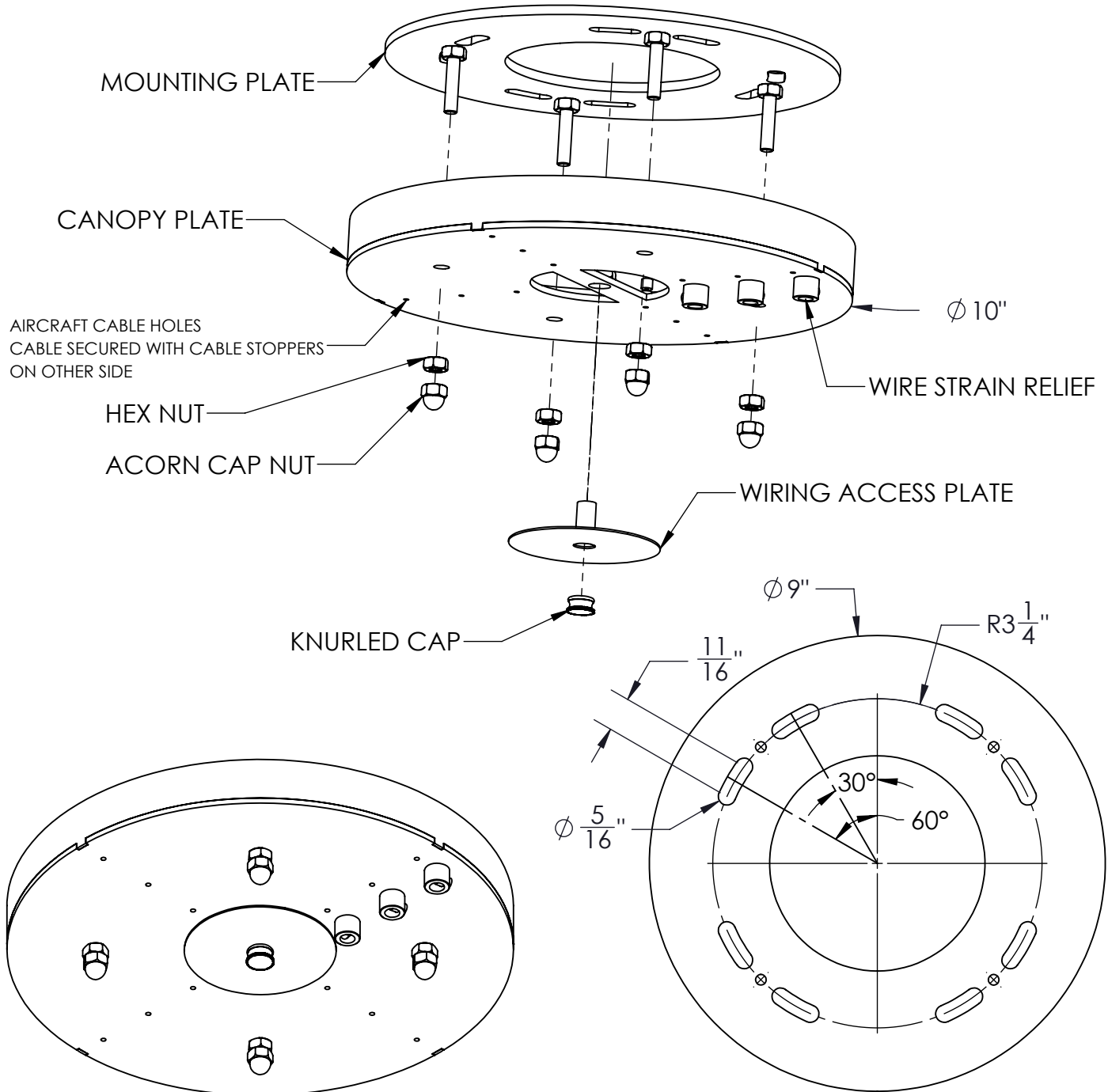
MOUNTING PLATE LAYOUT
