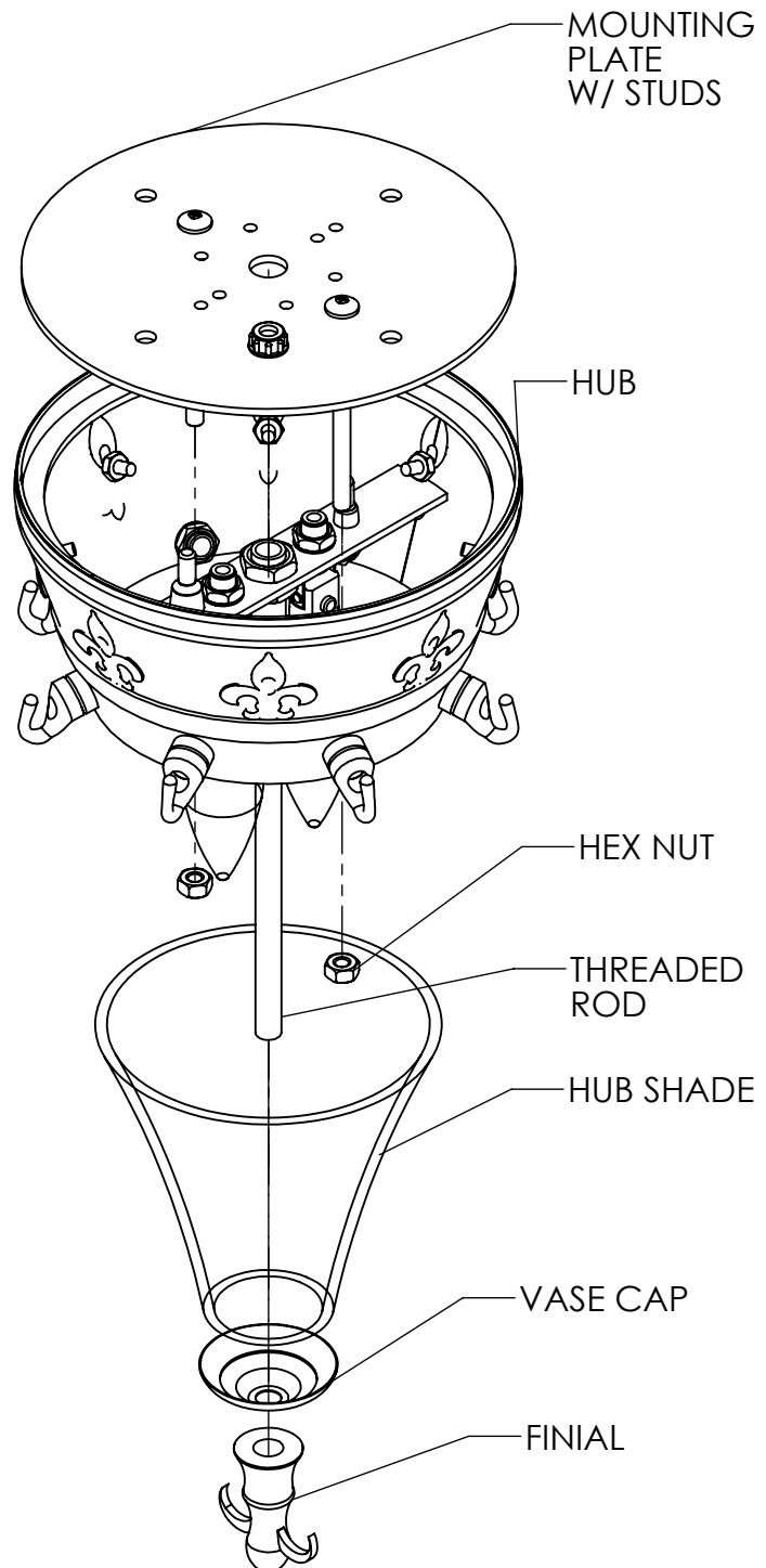
HUB ASSEMBLY
