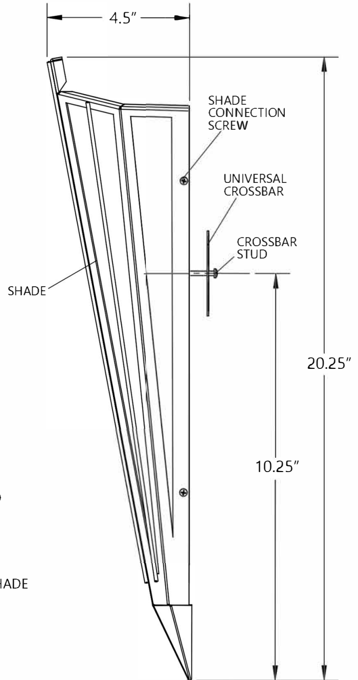
SIDE VIEW
