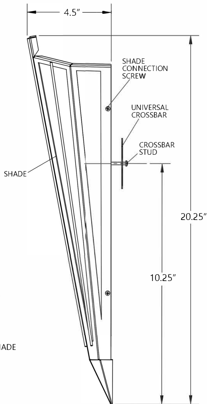
SIDE VIEW
