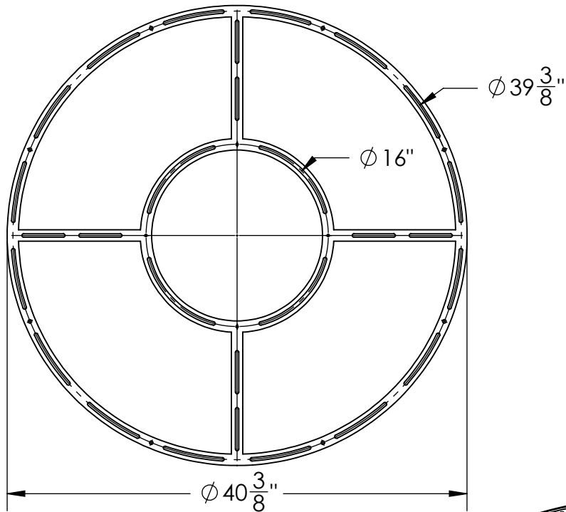
MOUNTING PLATE DIMENSIONS
