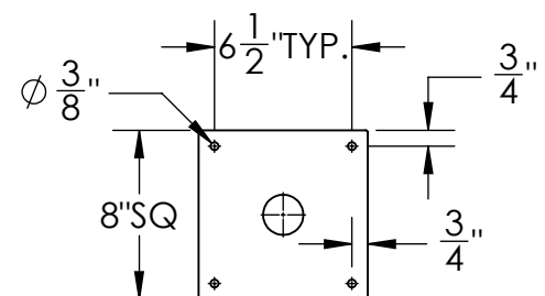
MOUNTING PLATE LAYOUT
