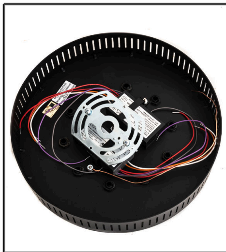
CANOPY INTERIOR DETAIL
