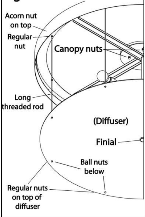
Bottom view
