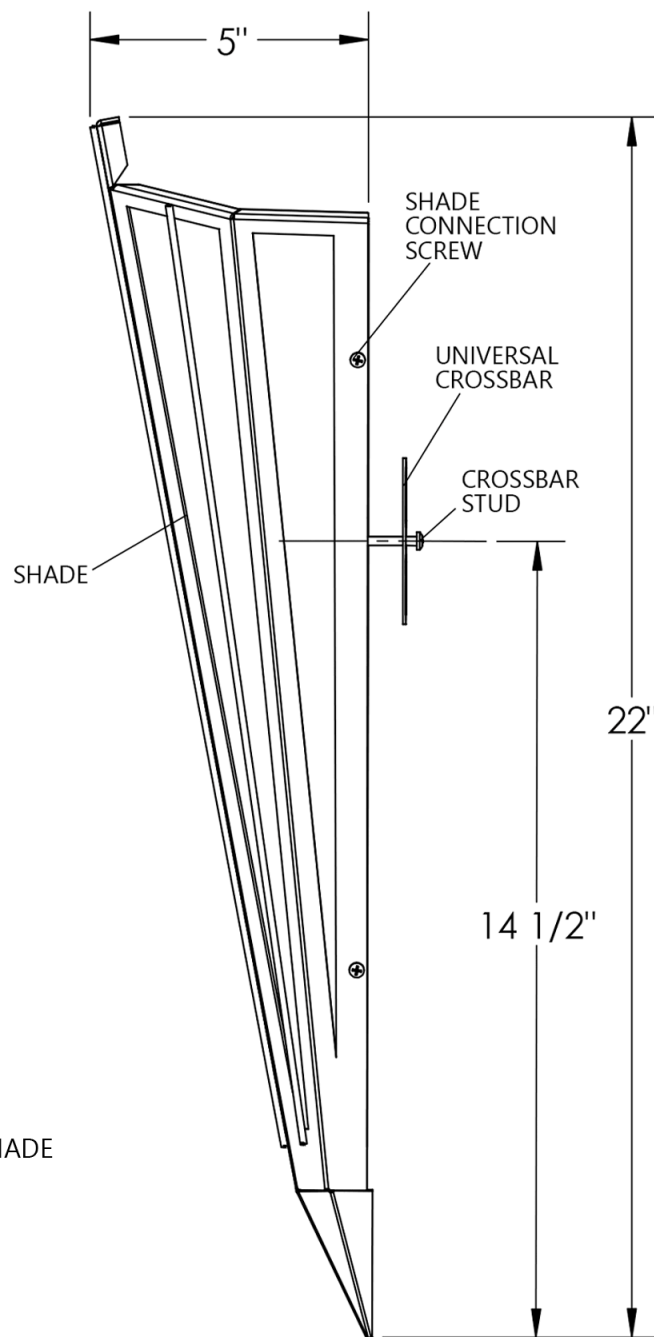
SIDE VIEW
